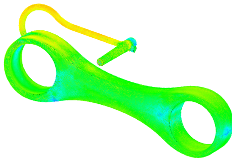
FIBER ORIENTATION
